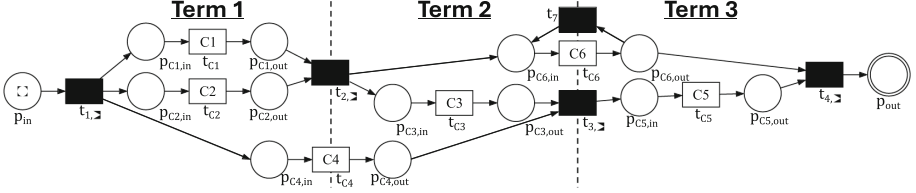
Fig. 3. Example workflow net N_1 .
